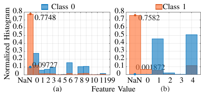
Fig. 3: Exemplary features (a) “ source_of_anc ” and (b) “ maternity_financial_assistance ” with different classwise imbalance in terms of availability of the data, Class 1 = live birth, Class 0 = stillbirth
