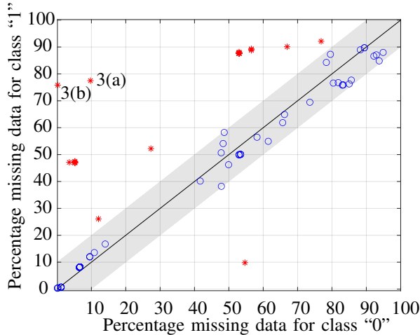
Fig. 4: Each data point ( *, \circ ) represents a feature with x and y coordinates being the missing percentage in class 0 and 1 respectively. Each feature outside the tolerance margins (marked as *) have high absolute percentage difference between the available class “0” and class “1”. As depicted, features from Figure. 3(a and b) are also apparently intolerable features
